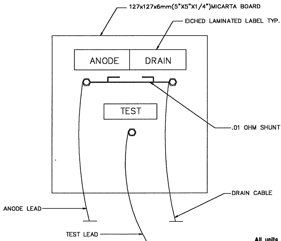
TEST TERMINAL BOARD DETAIL
