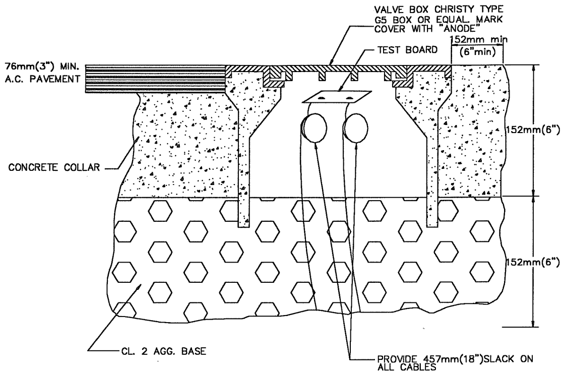
TEST STATION HOUSING DETAIL
