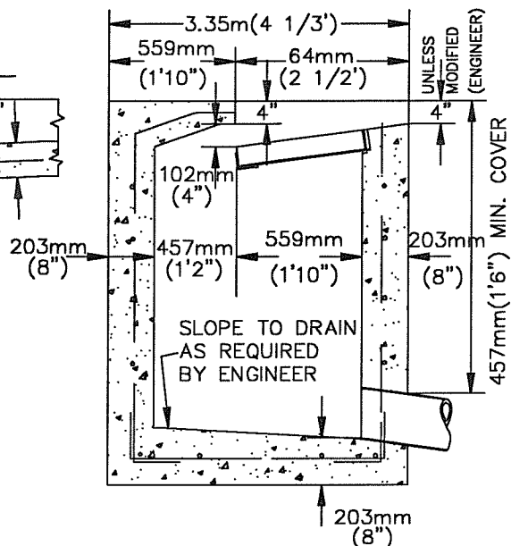
SECT. B-B
