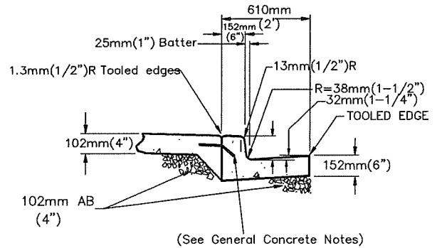
CURB AND GUTTER DETAIL
