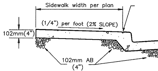
MONOLITHIC SIDEWALK, CURB AND GUTTER
