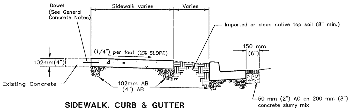
SIDEWALK, CURB & GUTTER WITH PLANTING STRIP
