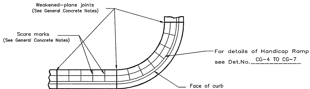
SIDEWALK AND CURB RETURN
