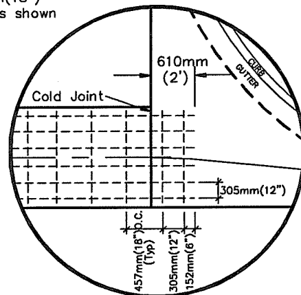
REBAR DETAIL
