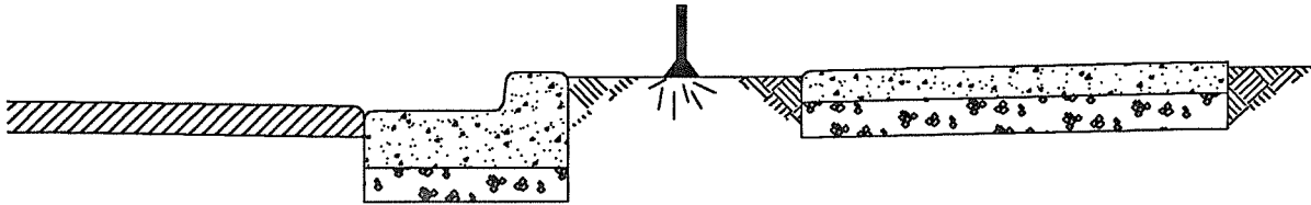
Sidewalk Standard (B)
