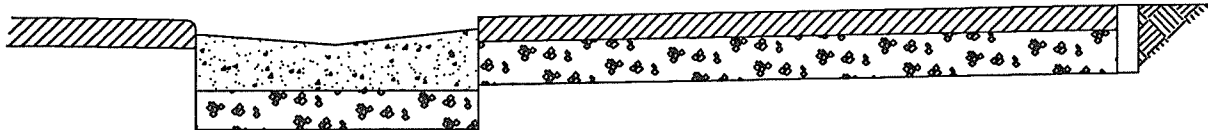
Parking Strip-Walkway Standard (C)
