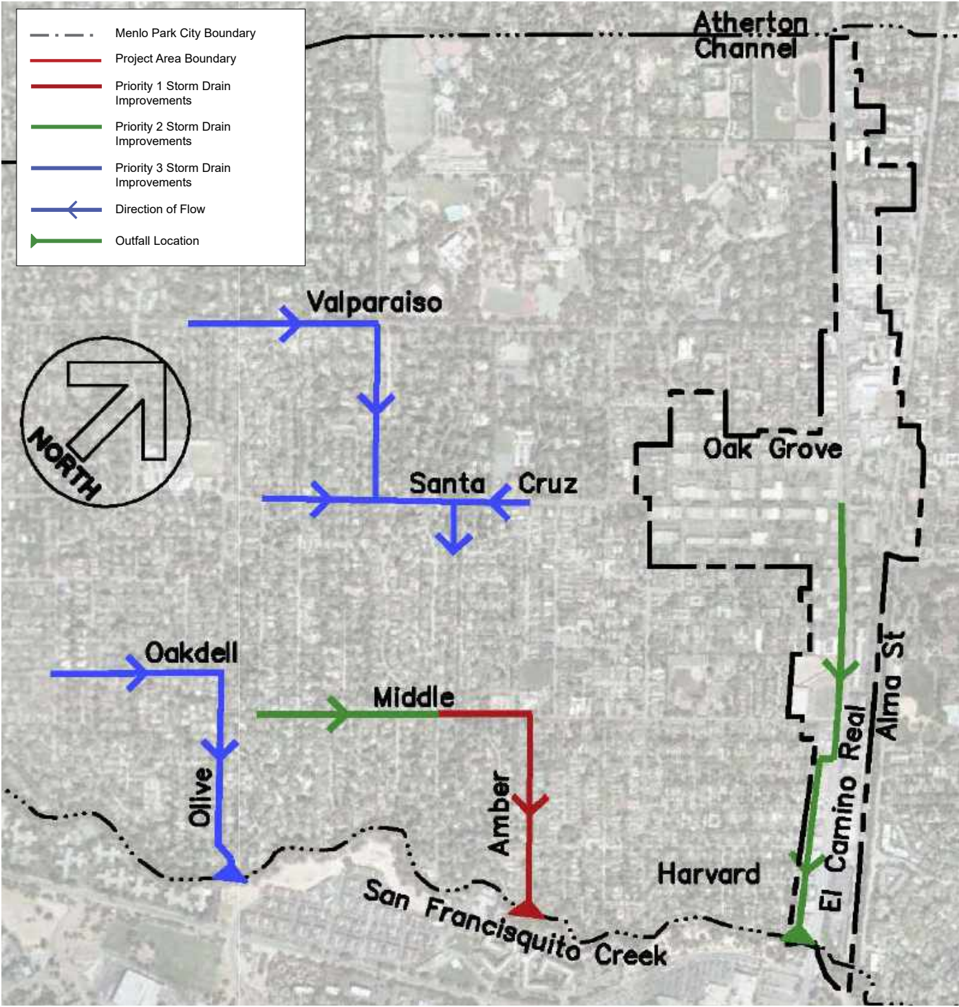
Figure G2. Storm Drainage
