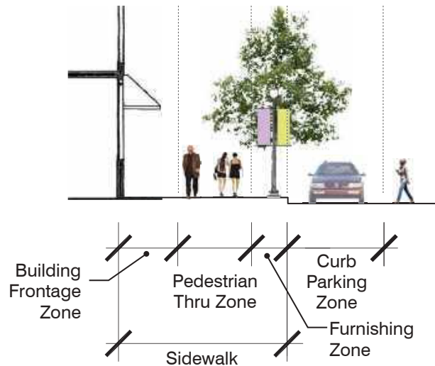
Figure D8. Sidewalk section. The qualities of the sidewalk may vary, but all should exhibit certain characteristics, including a Furnishings Zone, Pedestrian Thru Zone, and Building Frontage Zone (where possible)
