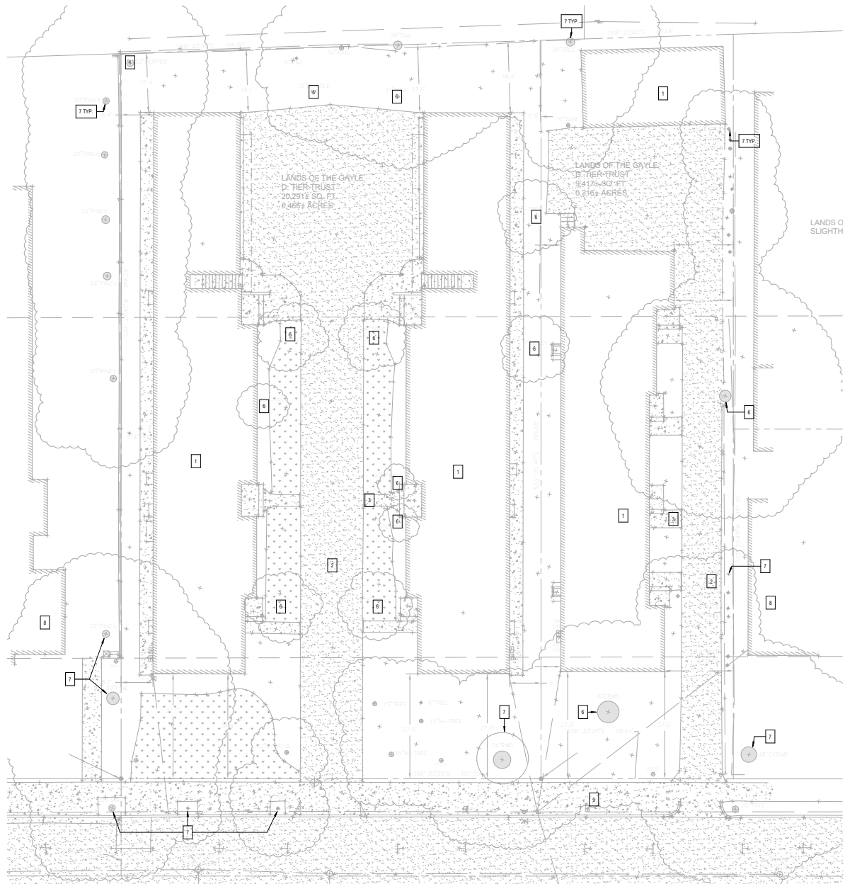
1 SITE PLAN DEMO 3/32" = 1'-0"
